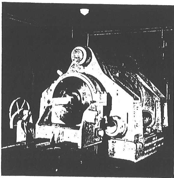
Large extrusion press for solventless cordite manufacture.
