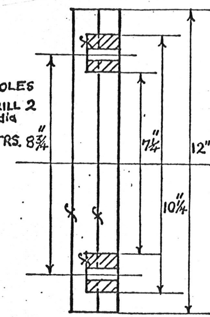
SECT. B-B
