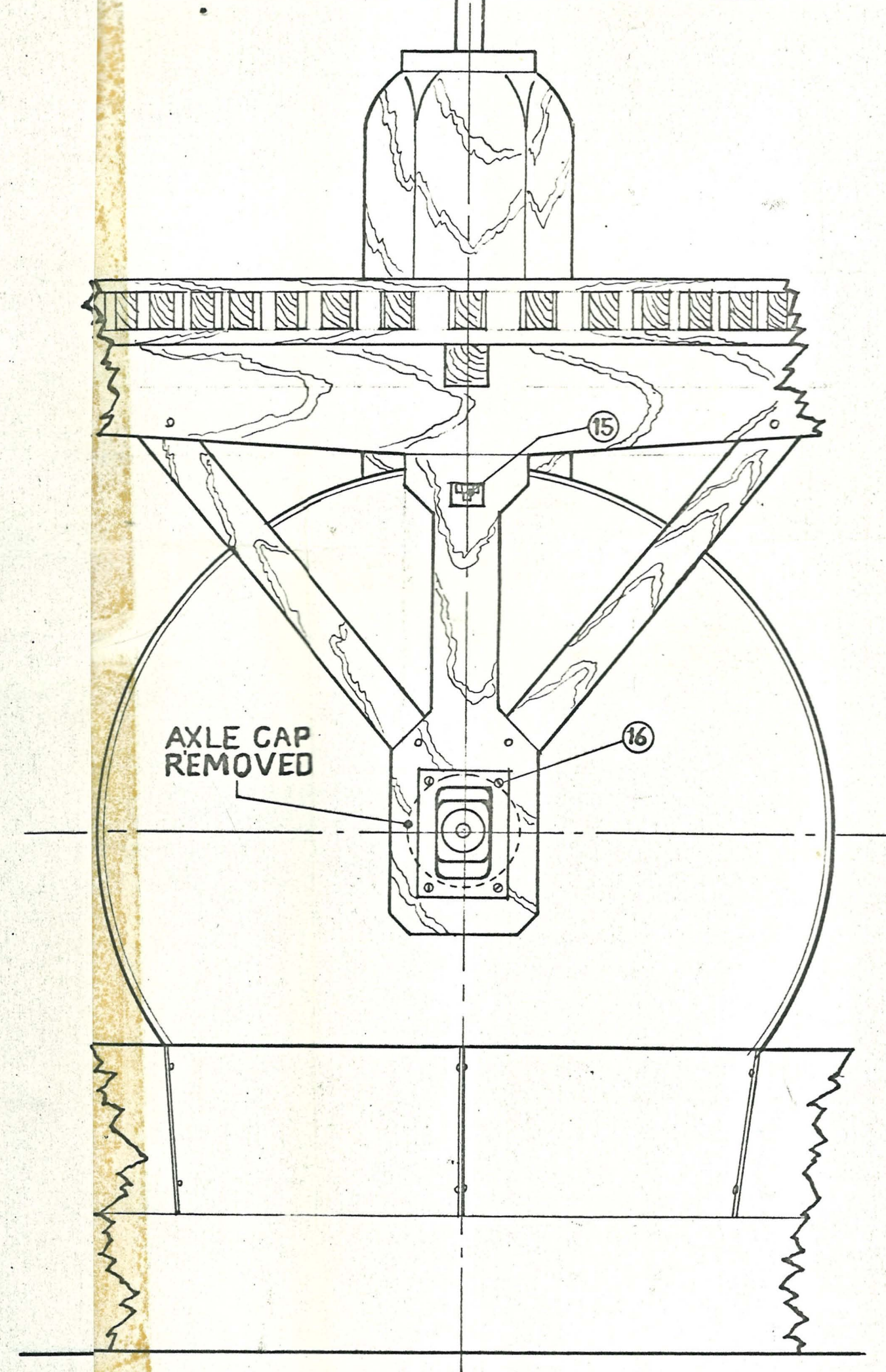
PART VIEW ARROW 'A' OUTERDRIVE BRACKETS
