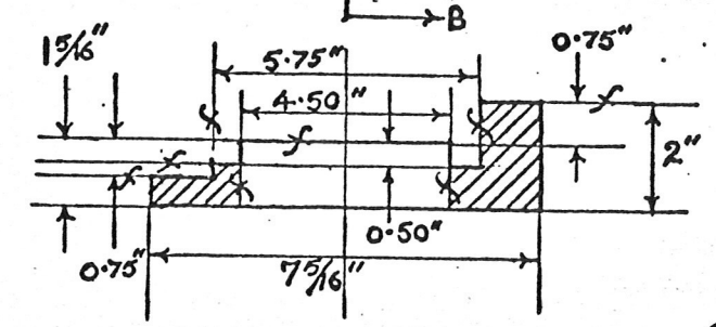
SECT. A-A
