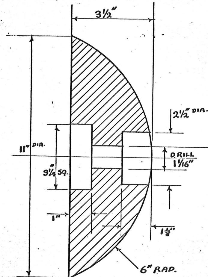
SECT. A-A
